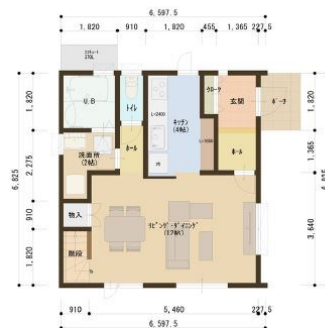
First floor plan 1 階
